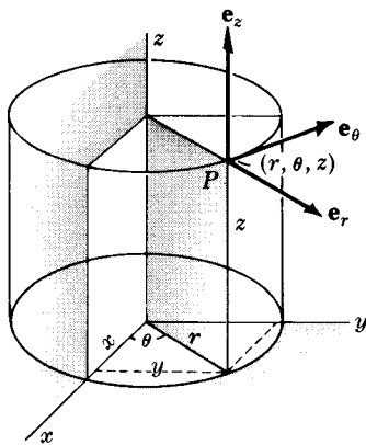
Fig. 22-12. Cylindrical coordinates.
